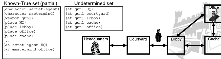
Fig. 3 Diagram of the secret agent world.
