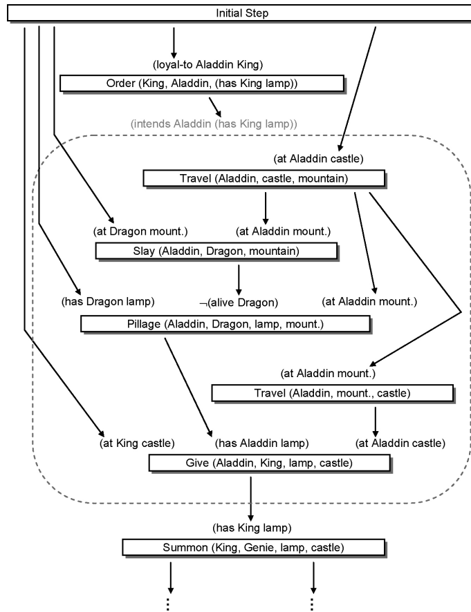
Fig. 2 Part of a narrative plan with intentionality.
