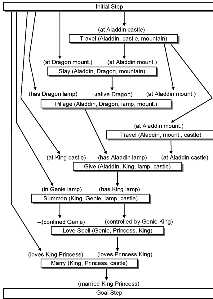
Fig. 1 A narrative plan generated by a conventional planner.
